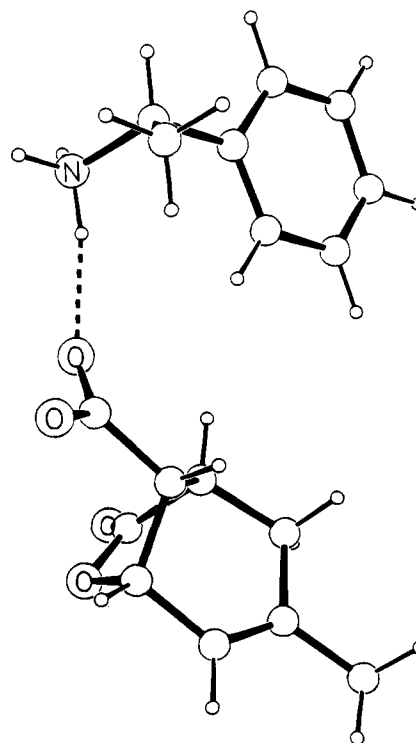
Figure 1. X-ray crystal structure of one of the two (S)-(-)- \alpha -methylbenzylamine salts of ( \pm )- 10 . The absolute configuration of the carboxylate in this diastereomer is opposite to that required for the synthesis of subunit A.
